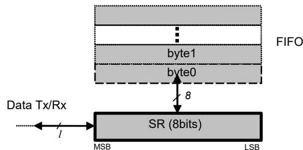
Figure 27. FIFO and Shift Register (SR)
